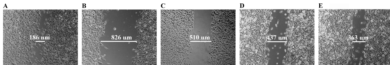
Figure 3. Effect of viscosin on migratory activity of the metastatic prostate cell cancer line PC-3M: (A) DMSO control (negative); (B) LY294002 control (positive) at 7.5 \mu\text{M} ; (C) viscosin at 20.0 \mu\text{M} ; (D) viscosin at 15.0 \mu\text{M} ; (E) viscosin at 10.0 \mu\text{M} .
