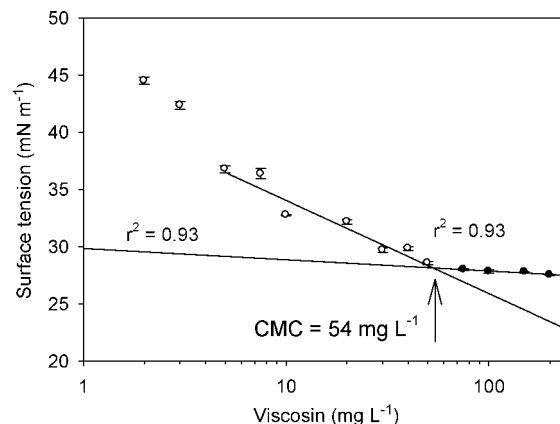
Figure 1. Effect of viscosin concentration on surface tension. The cmc was determined from the intersection of regression lines for (○) below cmc (5 to 50 mg L -1 ) and (●) above cmc (75 to 200 mg L -1 ). Each data point is the average and standard deviation of three replicate samples.
